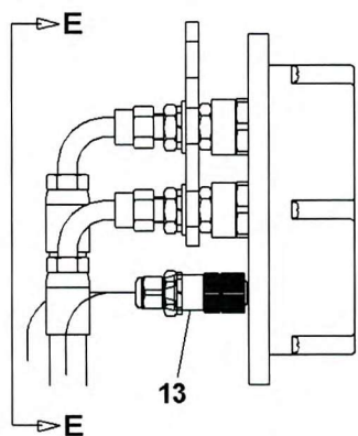
VIEW D-D
