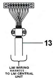
VIEW F-F
