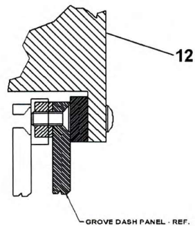
DETAIL 'C' NO SCALE
